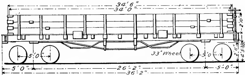
Fig. 69. Side Elevation.
